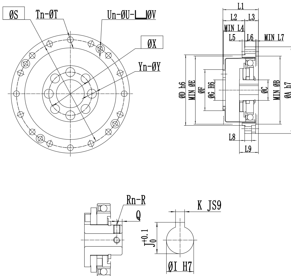
Wave generator shape for Model 14/17
